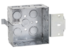
72171 MS 1/2 & 3/4 MS bracket for 1 5 / 8 ", 2 1 / 2 ", 3 3 / 8 ", 4" metal studs
