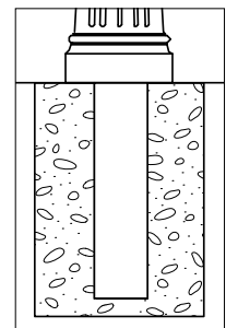
Direct In-ground Base Installation
